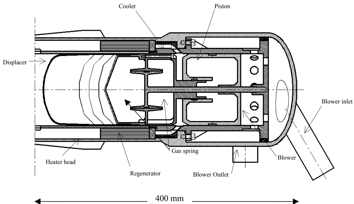
Figure 2. Single engine and blower (from opposed pair)
