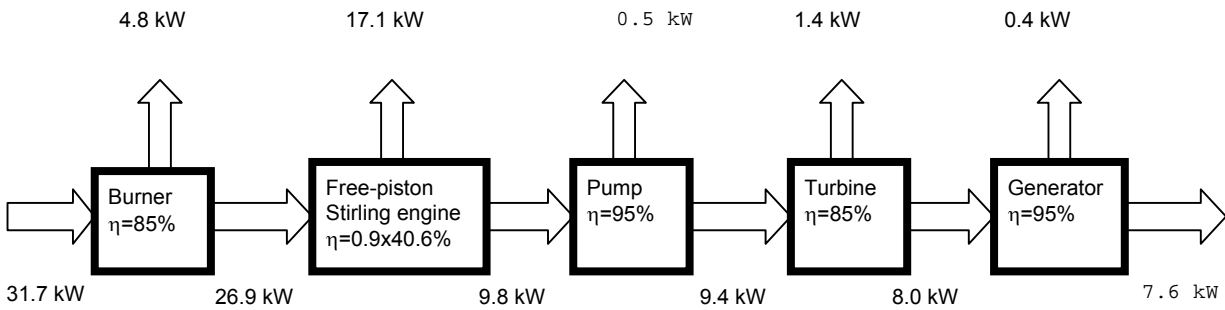
Figure 4. Design point system energy flows
