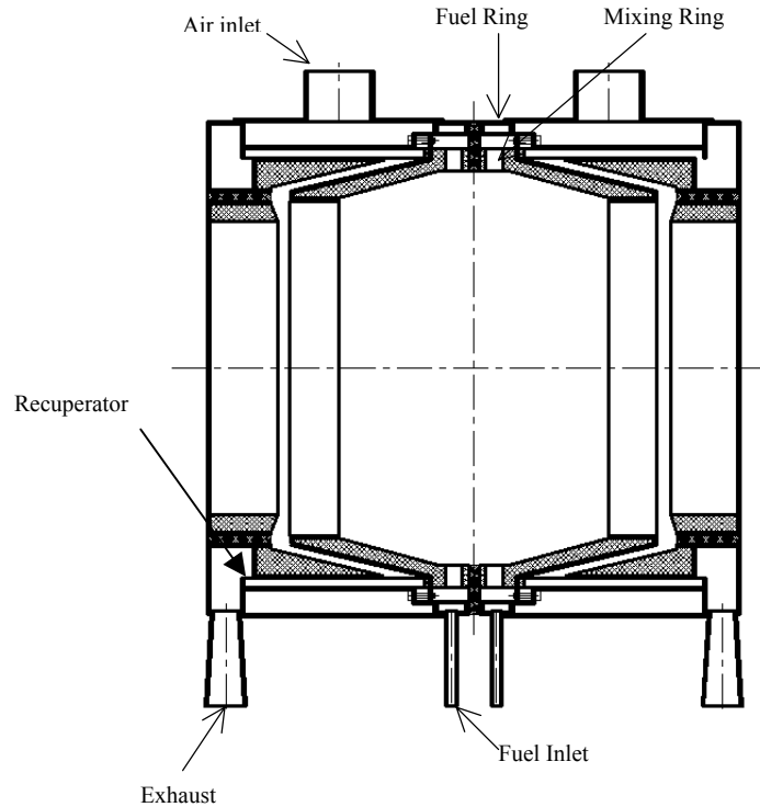
Figure 3. Burner layout
