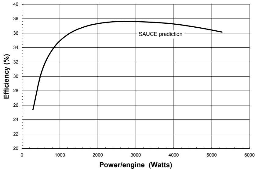
Figure 5. Simulated single engine performance at various powers
